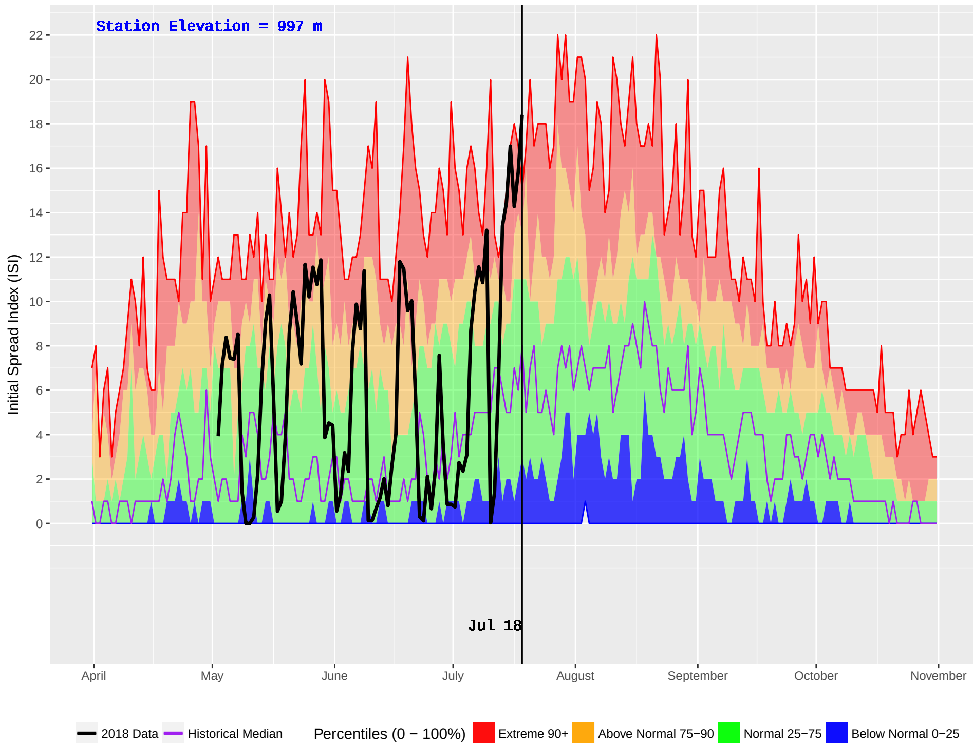
SMALLWOOD (404) : Historical (1991–2016) and Current (2018) Daily Initial Spread Index (ISI)
