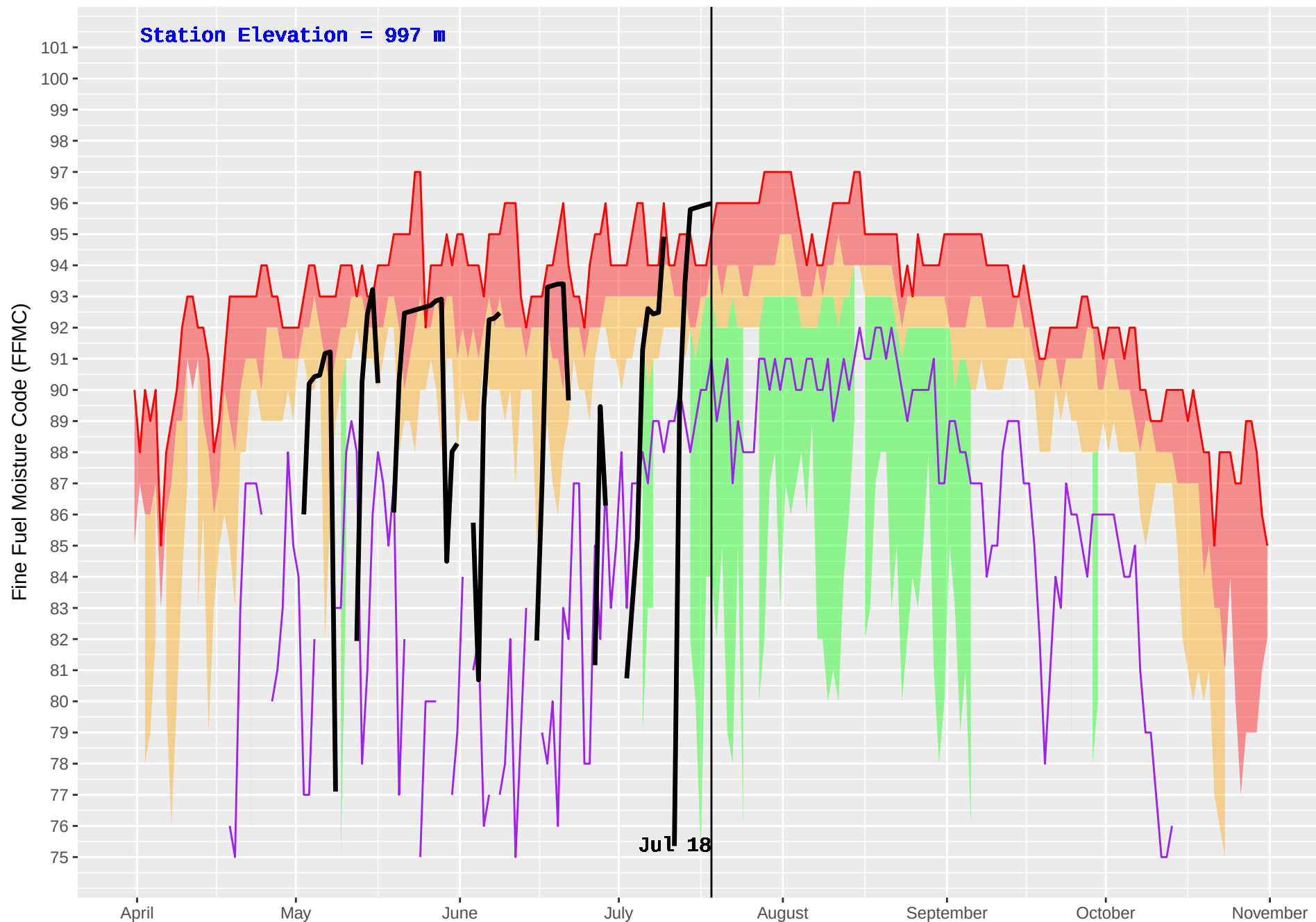
SMALLWOOD (404) : Historical (1991–2016) and Current (2018) Daily Fine Fuel Moisture Code (FFMC)
