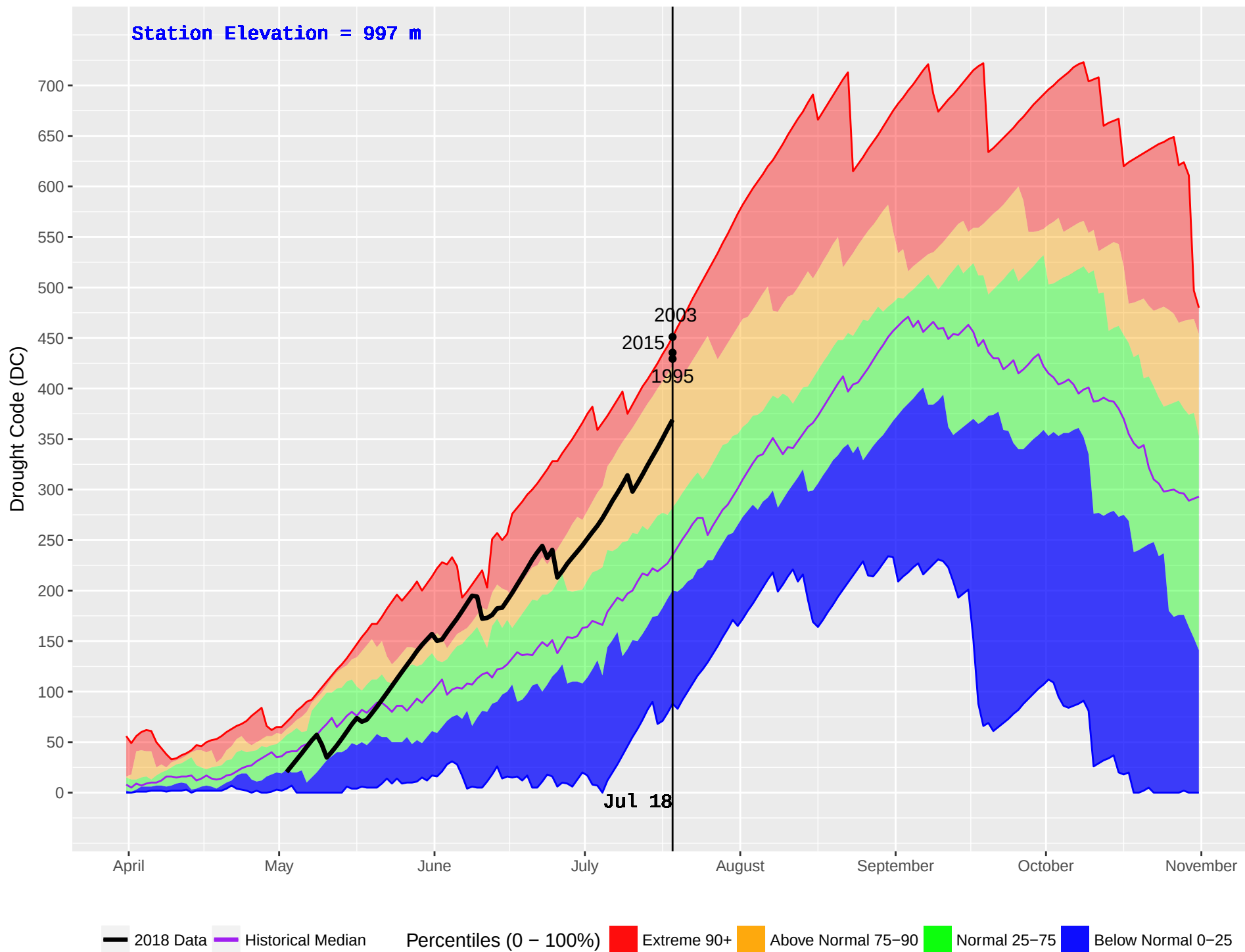
SMALLWOOD (404) : Historical (1991–2016) and Current (2018) Daily Drought Code (DC)
