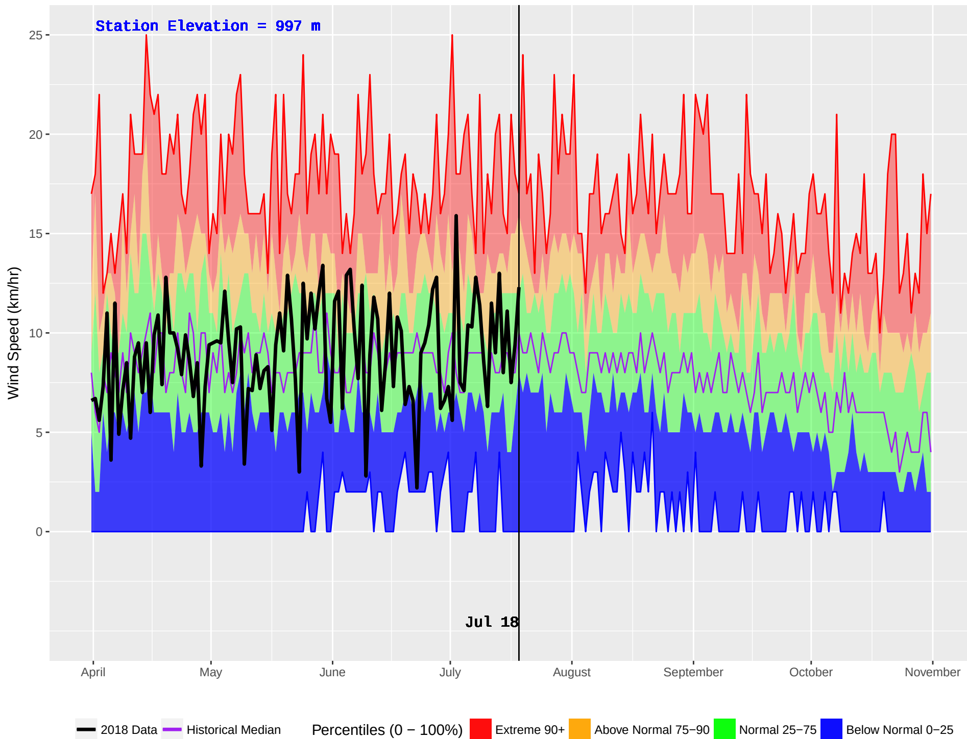
SMALLWOOD (404) : Historical (1991–2016) and Current (2018) Daily Wind Speed
