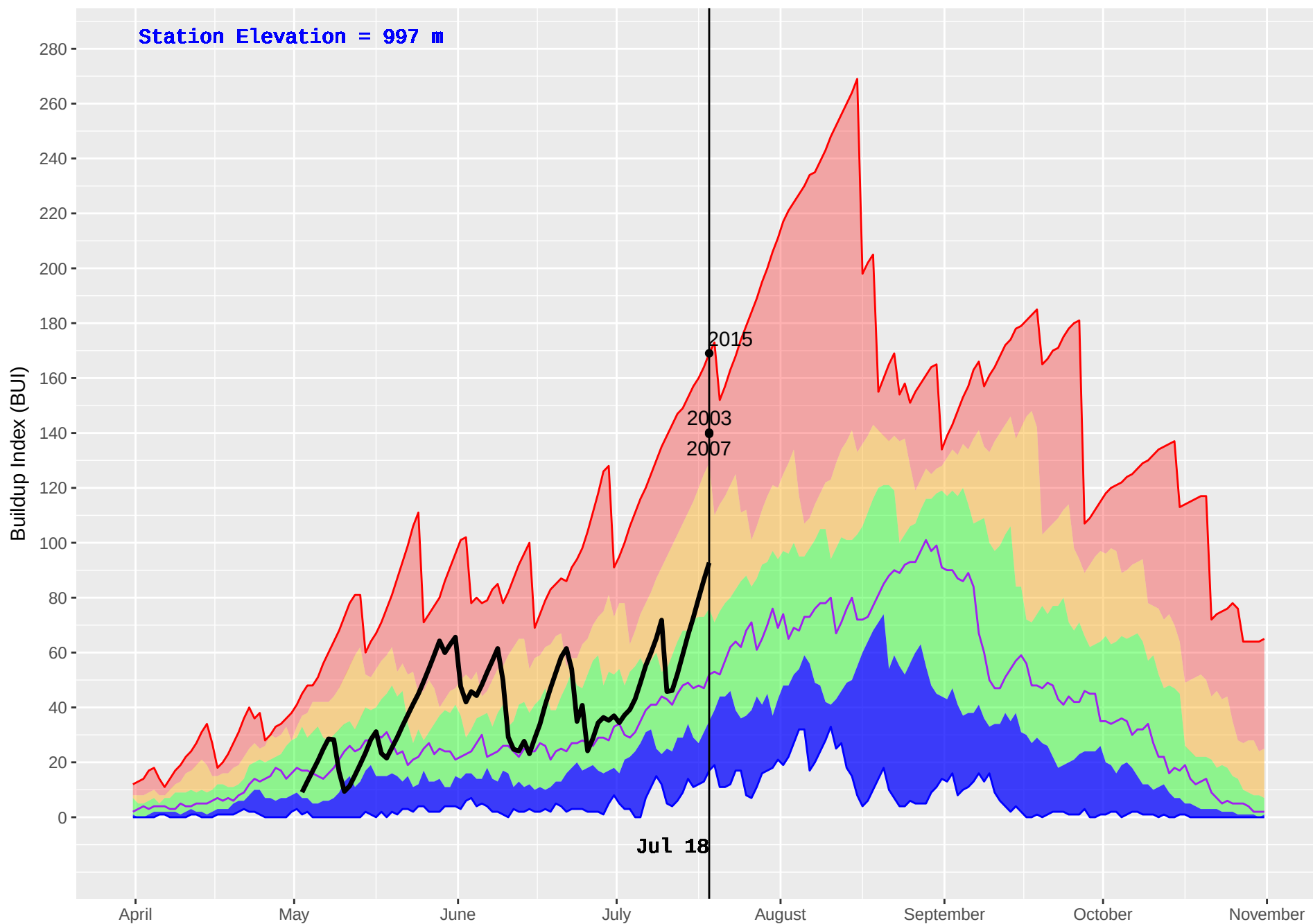
SMALLWOOD (404) : Historical (1991–2016) and Current (2018) Daily Buildup Index (BUI)
