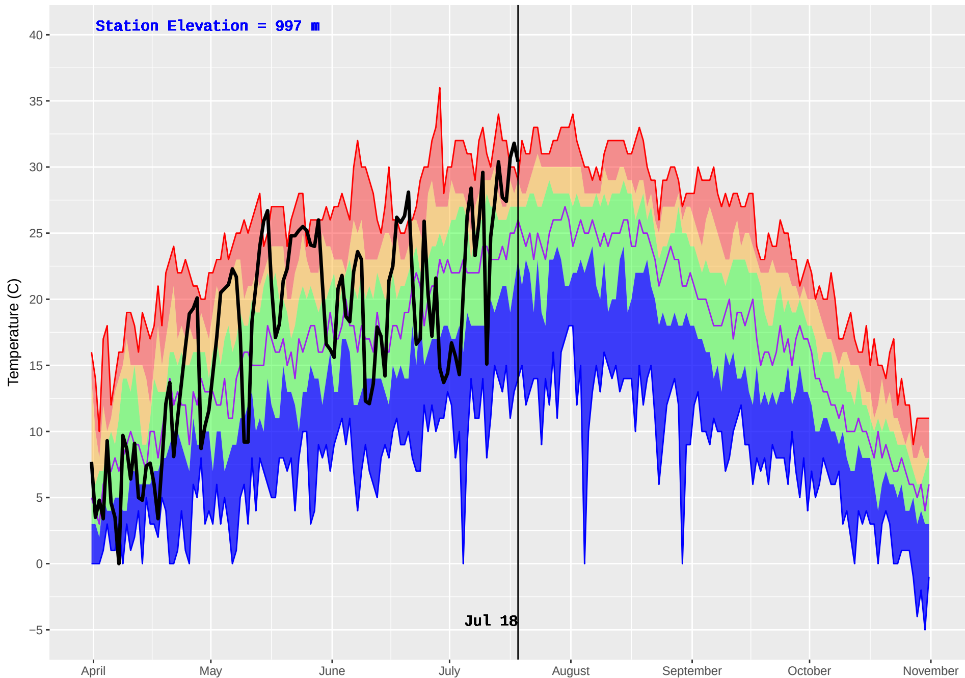
SMALLWOOD (404) : Historical (1991–2016) and Current (2018) Daily Temperature
