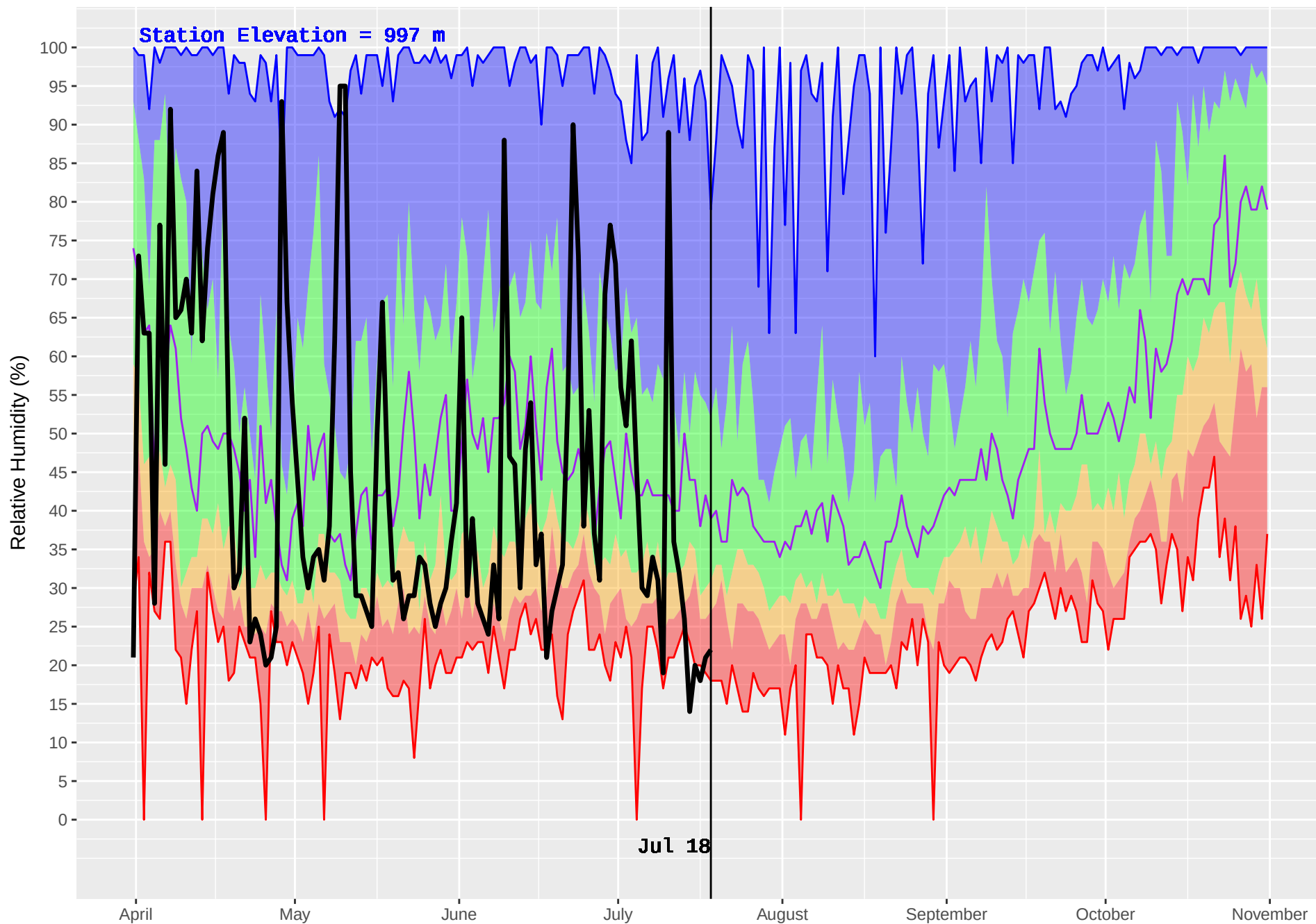
SMALLWOOD (404) : Historical (1991–2016) and Current (2018) Daily Relative Humidity
